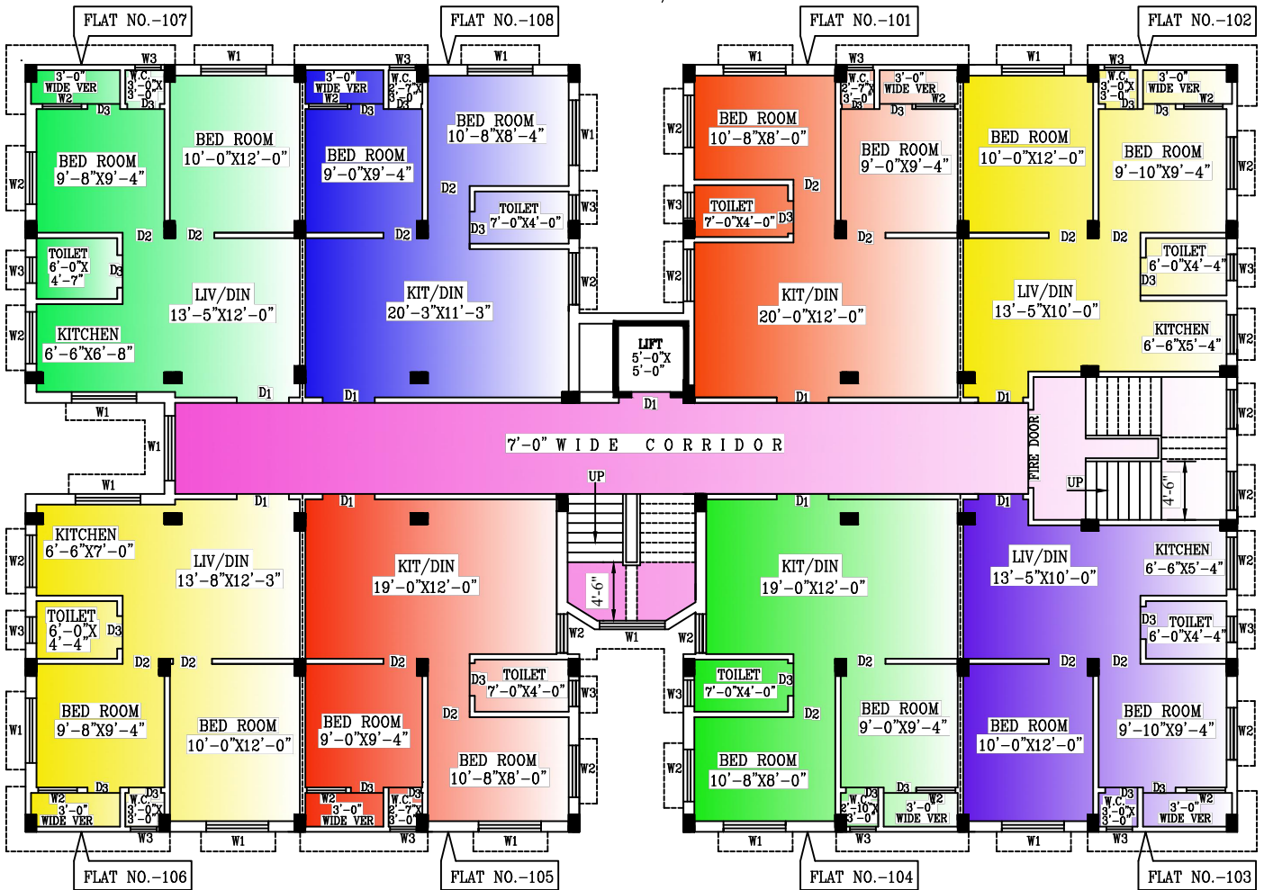
PROPOSED 1ST,2ND,3RD, 4TH & 5TH FLOOR PLAN BLOCK - A
